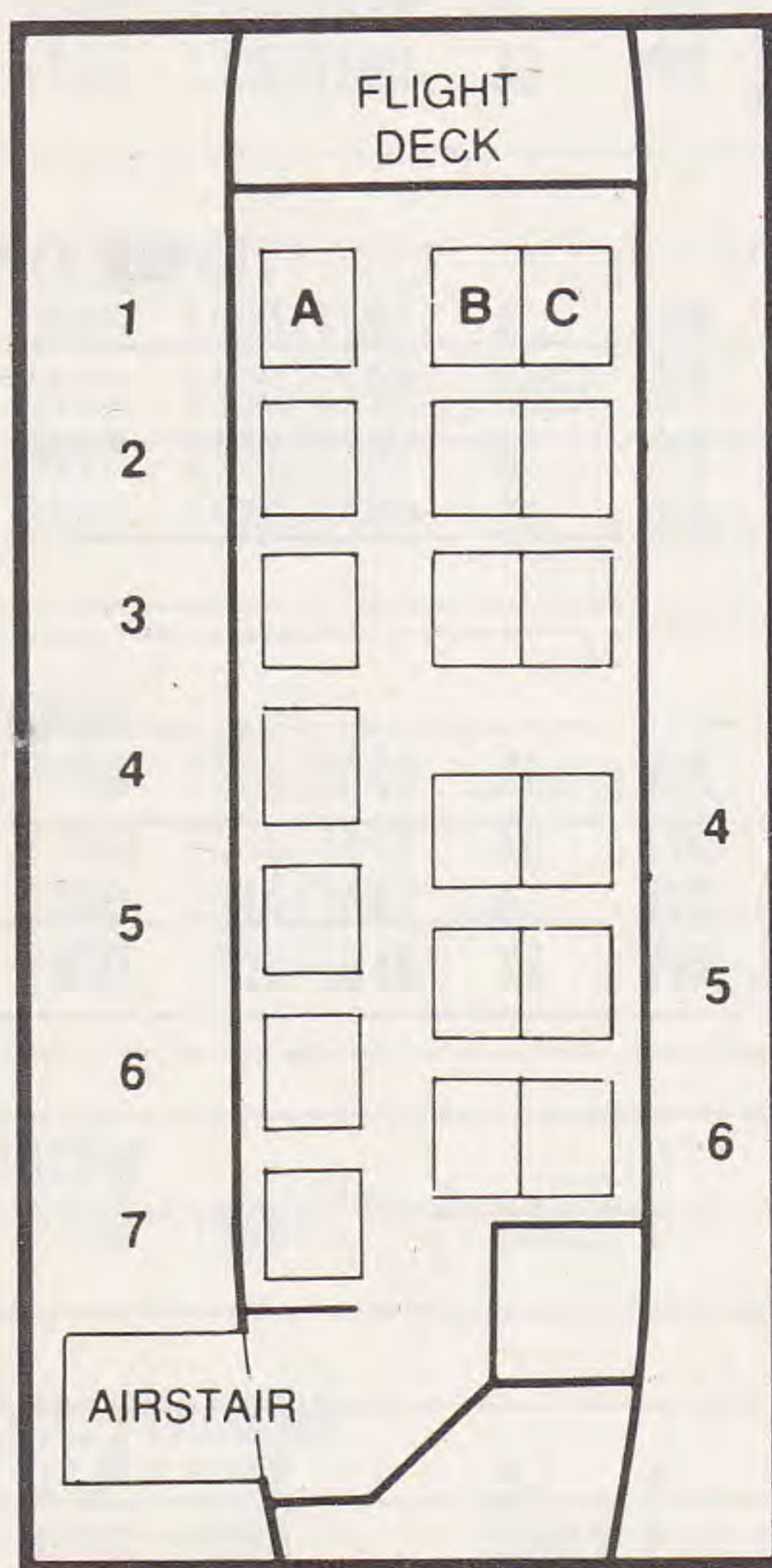
BAe Jetstream 31
