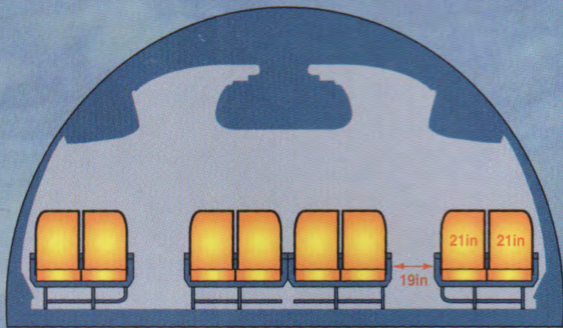
The Canada 3000 A330-200 Seat Configuration 8 abreast in 4 double seats with twin aisles
